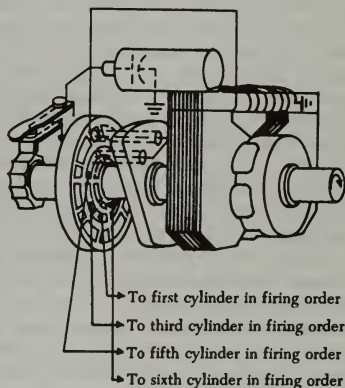
FIGURE 4-19. Brush-type distributor operation.
